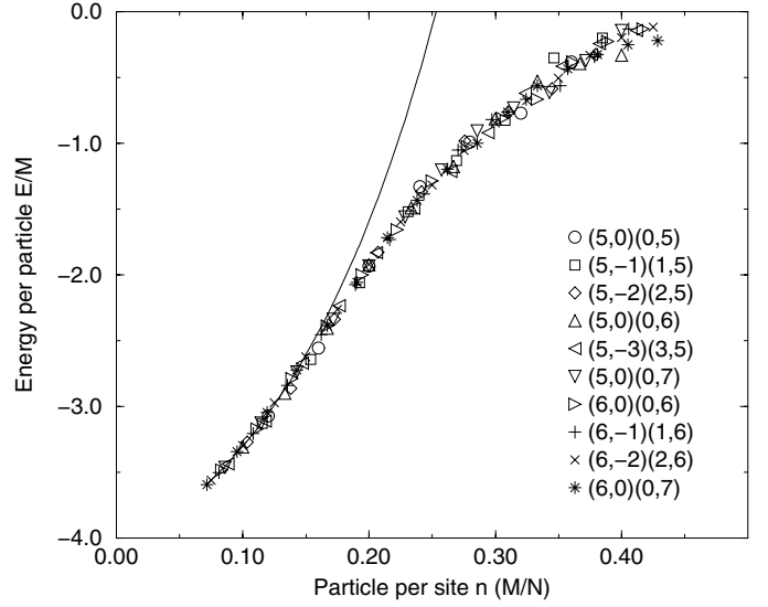
Fig. 14. Boson energy per particle E/M versus particle density M/N data for ten lattices and M \geq 3 . Data from different lattices collapse onto one curve. The solid line corresponds to the fitting function -4 + 4\pi n(A + B/|\ln(na^{*2})|) with a^* = 1.36 , A = -0.016 , and B = 0.959 , which is equation (5.4) with parameters from Table 6.
