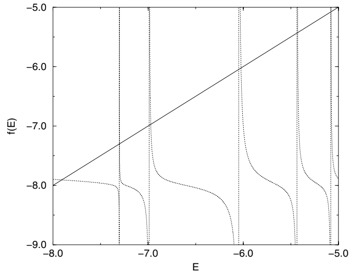
Fig. 3. f(E) = E_0 + T_1(E) versus E for 10 \times 11 lattice with \mathbf{P} = (0, 0) and E_0 = -8.0 (i.e., E_0 = \mathcal{E}(0) + \mathcal{E}(0) .) The intersections with the line y = E are the exact two-particle energies.
