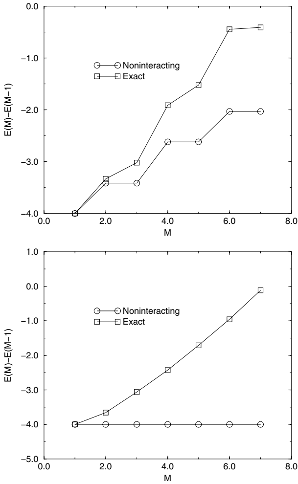
Fig. 8. Shell effect for 5 \times 8 lattice (fermion, top graph; boson, bottom graph). Exact, interacting groundstate energies are compared with noninteracting energies for up to seven particles. Energy increment E(M) - E(M - 1) is shown.
