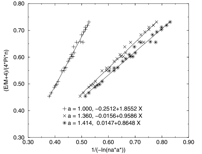
Fig. 15. (E/M + 4)/(4\pi n) versus 1/|\ln(na^{*2})| plot to check Schick's formula for two-dimensional dilute bosons (Eq. (5.3)). The data points are for M \geq 3 and n \leq 0.15 from those in Figure 14, for lattices from 5 \times 5 to 6 \times 7 . For the three a^* values, the a^* = 1.36 choice gives A = -0.016 \approx 0 and B = 0.959 \approx 1 .
