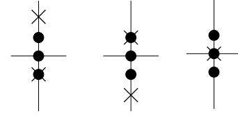
Fig. 10. Momentum space exclusions in t-matrix M = 3 calculation for the state (0,0)(0,1)(0,-1) . The crosses indicate exclusions when calculating pair energy for (0,0)(0,1) (left figure), (0,0)(0,-1) (middle), and (0,1)(0,-1) (right) respectively.
