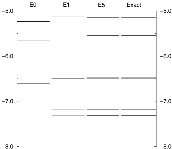
Fig. 7. Two-fermion energy levels for the 10 \times 11 lattice with \mathbf{P} = (0, 0) . From left to right, the lowest few noninteracting energies E_0 , first t-matrix iteration E_1 , fifth t-matrix iteration E_5 , and the exact energy E_{\text{exact}} are plotted. Note that the third noninteracting energy from the bottom is doubly degenerate (see Tab. 2).
