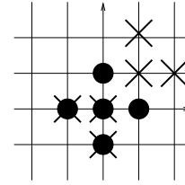
Fig. 12. Momentum space exclusions in t-matrix M = 5 calculation for momentum vectors \mathbf{q}_2 = (0, 1) and \mathbf{q}_4 = (1, 0) (dots without crosses). These two fermions are excluded from scattering into momenta from the set \bar{Q}^{2,4} (marked by crosses). The ground state is shown, with occupied momenta (0, 0) , (0, 1) , (0, -1) , (1, 0) , and (-1, 0) (solid dots).
