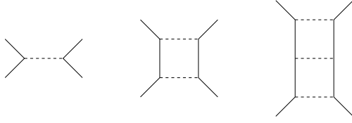
Fig. 16. The three figures represent perturbative terms involving V(\mathbf{q} - \mathbf{q}') , T_2(E, \mathbf{P}; \mathbf{q}, \mathbf{q}') and T_3(E, \mathbf{P}; \mathbf{q}, \mathbf{q}') . The t-matrix, T(E, \mathbf{P}; \mathbf{q}, \mathbf{q}') , is the sum of all these terms, i.e., it is the sum of the ladder diagrams to infinite order.
