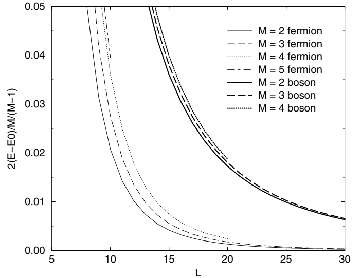
Fig. 1. Boson and fermion 2(E(M, L) - E_0(M, L)) / (M(M-1)) versus L for M = 2, 3, 4, 5 . All curves appear to converge at large L . The fermion (p-wave) result is much less than the boson result (s-wave). The M = 4 plot goes to L = 20 and the M = 5 plot to L = 10 . The boson M = 5 curve is too high to be included in this plot.
