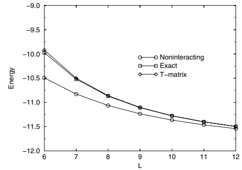
Fig. 13. Noninteracting, t-matrix, and exact energies for M = 3 , \mathbf{P} = (0,0) ground state (0,0)(0,1)(0,-1) on a series of L \times (L+1) lattices as a function of L .
