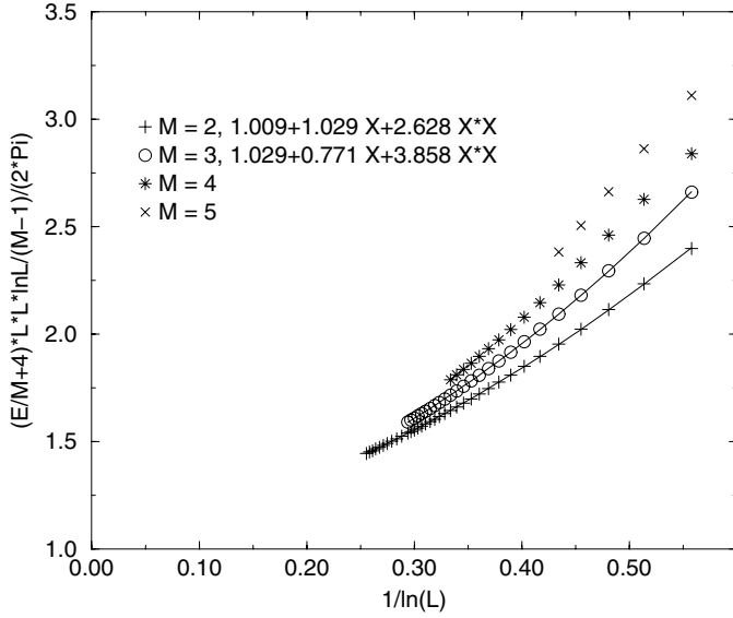
Fig. 2. Boson (E(M, L) + 4M)L^2 \ln L / (2\pi M(M-1)) versus 1/\ln L for M = 2, 3, 4, 5 . Quadratic polynomial fitting is done for M = 2 and M = 3 . The fitted constant coefficients are approximately one, and the other coefficients from M = 2 and M = 3 are comparable.
