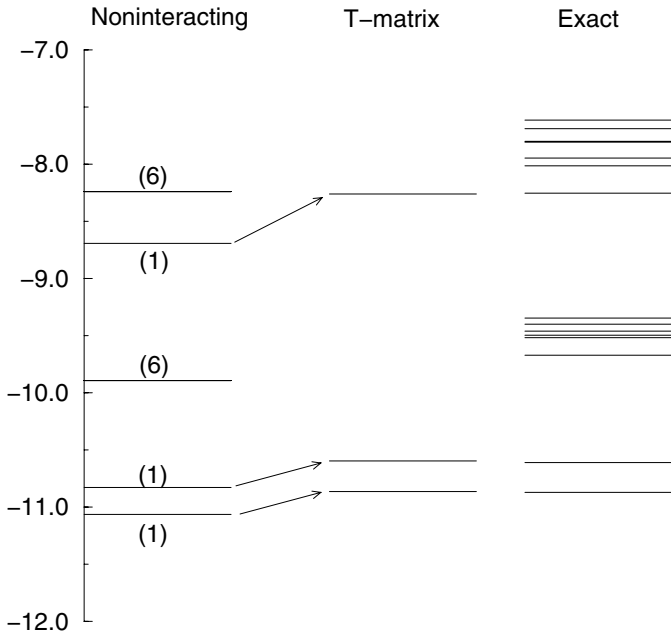
Fig. 11. Noninteracting, t-matrix, and exact energies of the three-particle fermion system on the 8 \times 9 lattice with \mathbf{P} = (0, 0) . The bracketed numbers refer to the degeneracies of the level (see Fig. 9). The arrows associate the noninteracting states with the t-matrix results. We have worked on nondegenerate noninteracting states so far.
