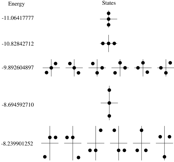
Fig. 9. Lowest five noninteracting energy levels for the 8 \times 9 lattice with M = 3 fermions and total momentum \mathbf{P} = (0, 0) . States in momentum space are drawn.
